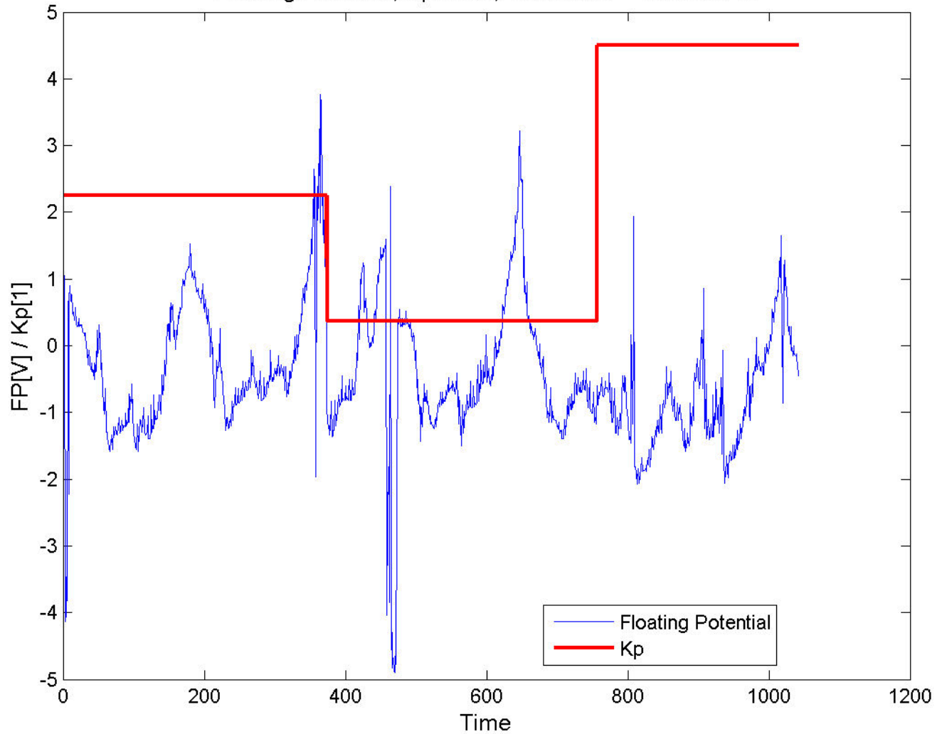
Floating Potential, Kp index, 12/07/2012 - 16/07/2012
