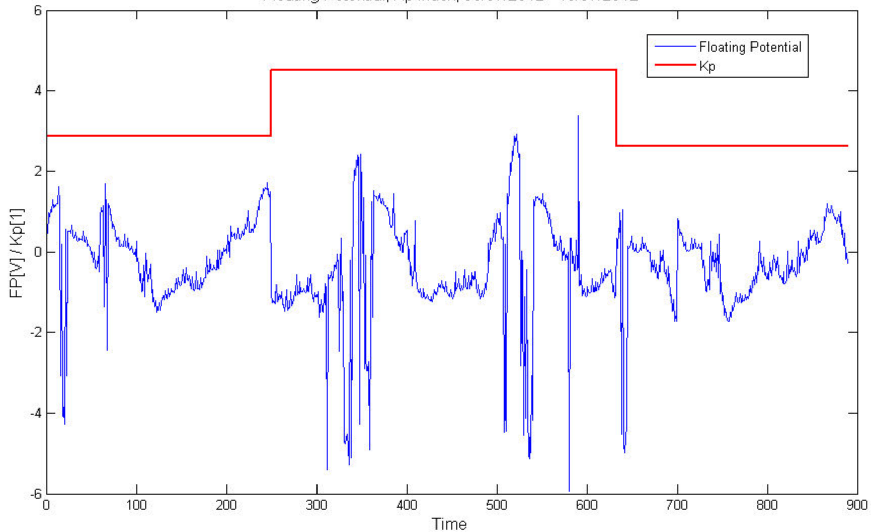
Floating Potential, Kp index, 06/07/2012 - 10/07/2012
