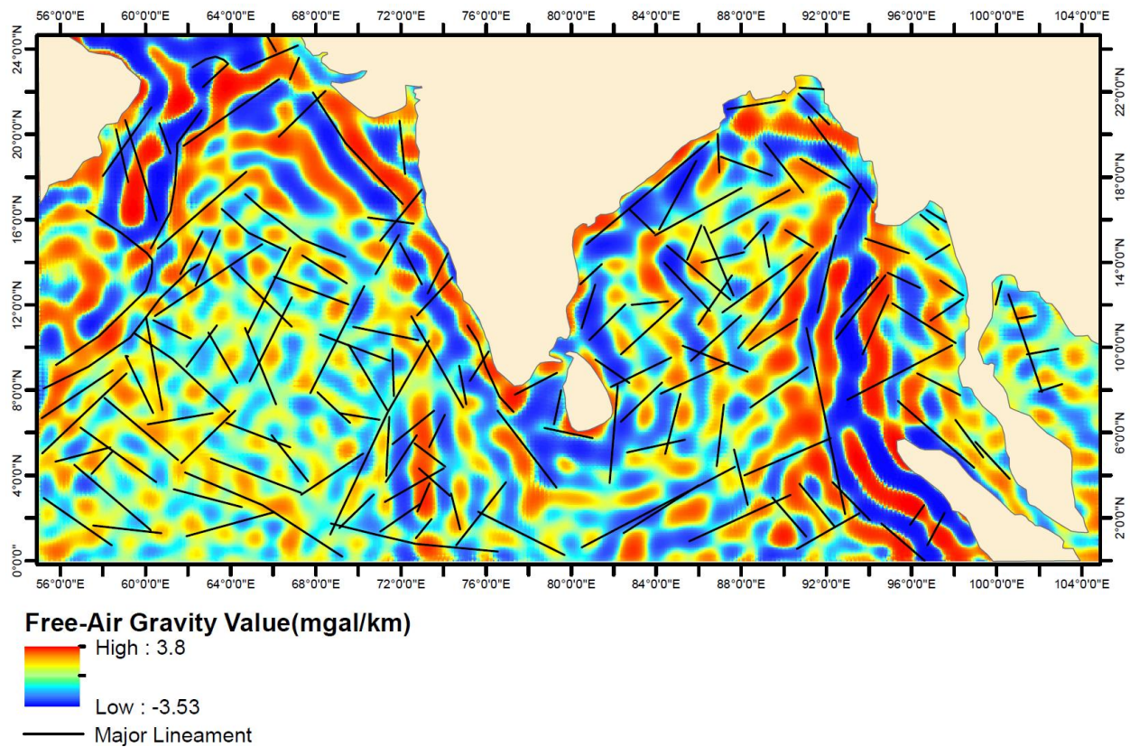
Figure 1: First Vertical derivative of Free-Air gravity anomaly generated over the Indian Ocean using GOCE satellite data. Major lineaments marked by Majumdar et al. (1998) have been overlaid on the enhanced Free-Air gravity anomaly Map. It clearly indicates that a numbers of additional lineaments could be delineated from the present enhanced anomaly map.
